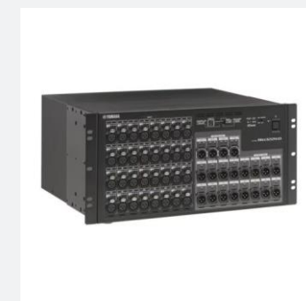
Yamaha Rio3224-D2
